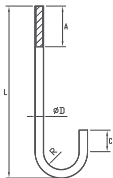
"J" SHAPE
