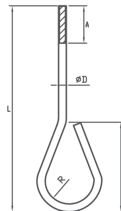
EYE SHAPE
