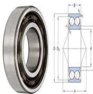
Ball bearing
