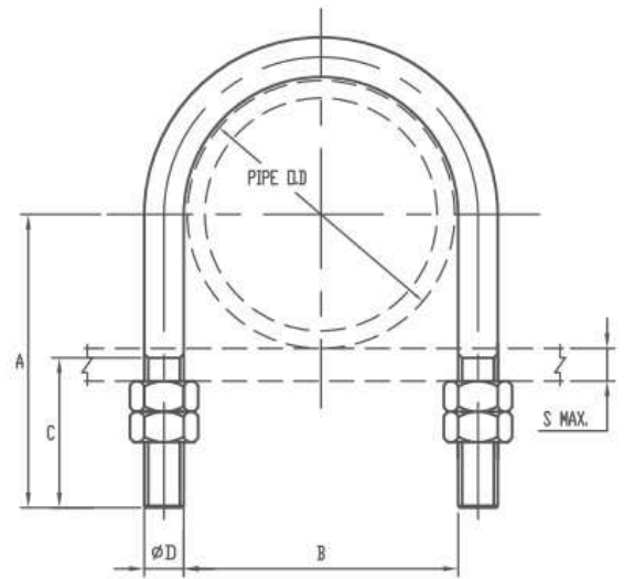
GRIP TYPE U-BOLT
