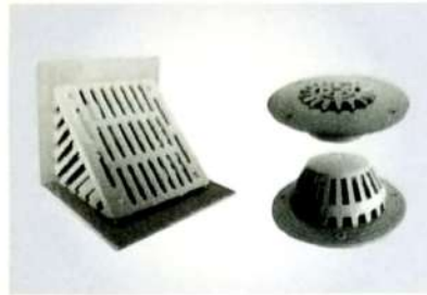
ART-99 UPVC Rain Water Outlet Size 3" & 4" Doom Type & Flat From UK & UAE
