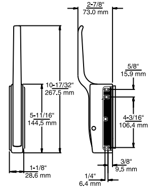
170 DIE-CAST OFFSET HANDLE
