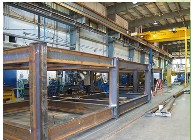
Structure Fabrication
