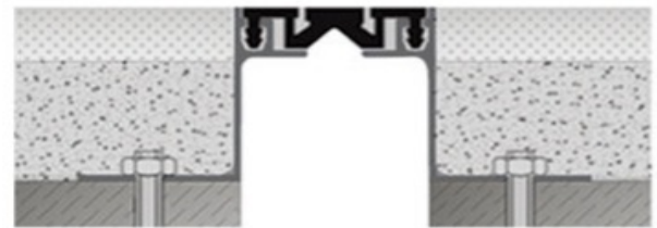
Floor Expansion Joint
