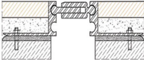
All Metal Expansion Joint
