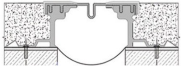
Waterproof 5000 Series HD
