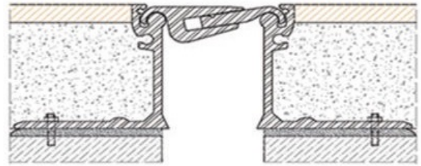
All Metal Expansion Joint
