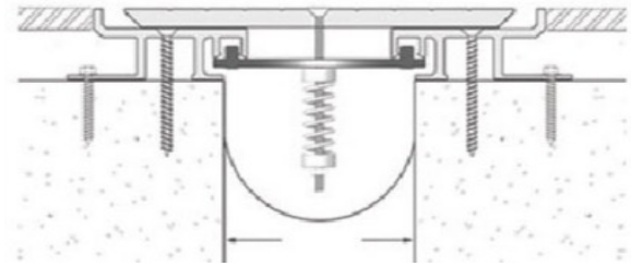
Seismic HD Parking EJ
