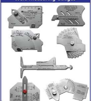
Weld Measuring Gauges
