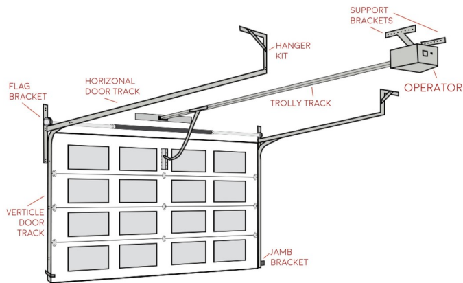
Automatic garage door mechanism
