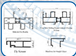
Insulated Thermal Break Gulf Extrusion
