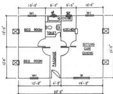
TWO BED ROOM VILLA
