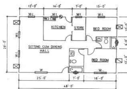
TWO BED ROOM VILLA
