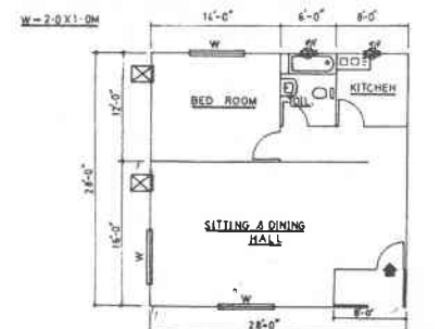
ONE BED ROOM VILLA
