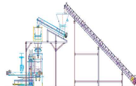
Auger filling machine
