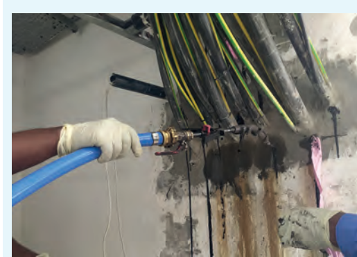
Sealing of Pipe Penetration
