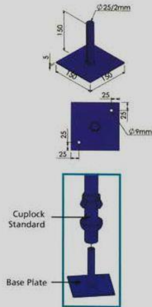
Base Plate
