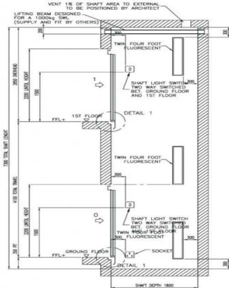
Side Vertical Section
