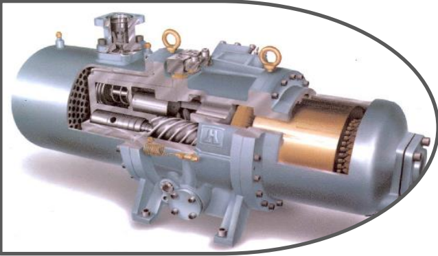
Screw compressors
