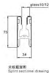
SA8900B-2B 上门夹 75mm top rail with pivot point
