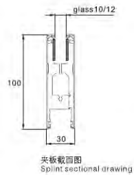
SA8900B-2A 上门夹 100mm top rail with pivot point
