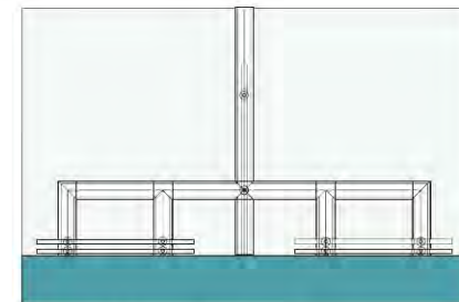
单边分体收纳布局(左向, 右向, 或双向收纳) Unilateral fission receive layout (left to right to, or two-way receive)
