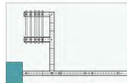
墙体外露式收纳布局(左向, 右向, 或双向收纳) Wall exposed to receive layout (left to right to, or two-way receive)
