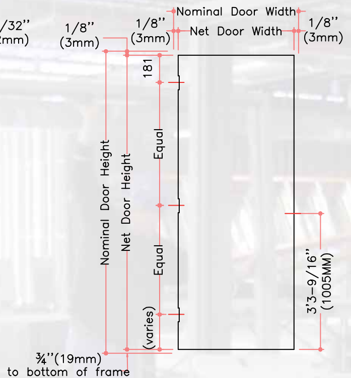
Single Door Elevation
