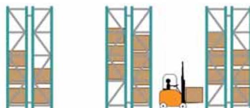
Standard Pallet Rack Configuration
