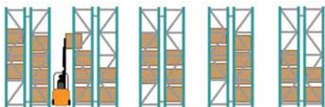
Very Narrow Aisle Pallet Rack Configuration
