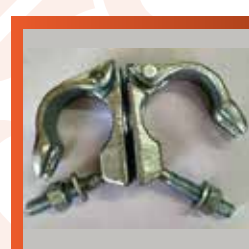
Swivel Coupler
