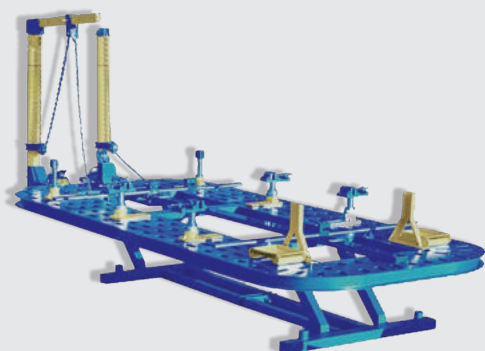
Body Pulling Bench
