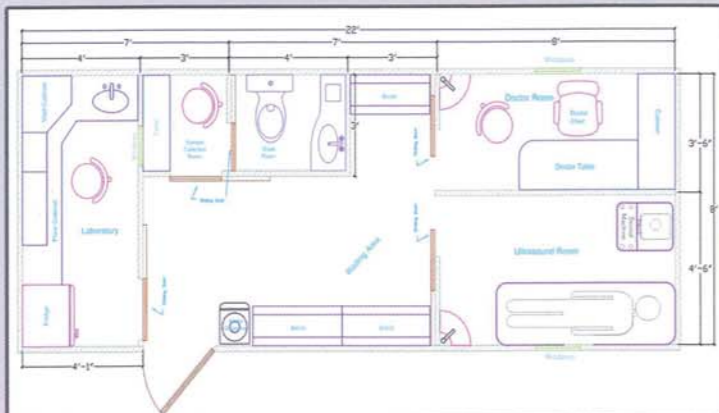
Floor Plan
