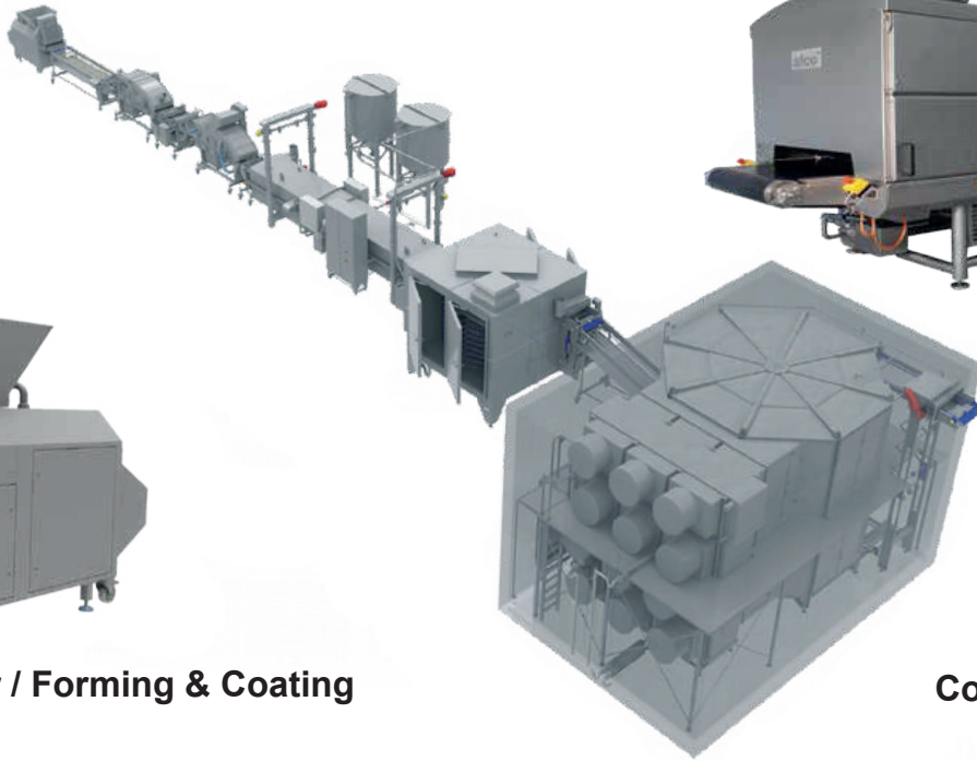
Contact Cooking
