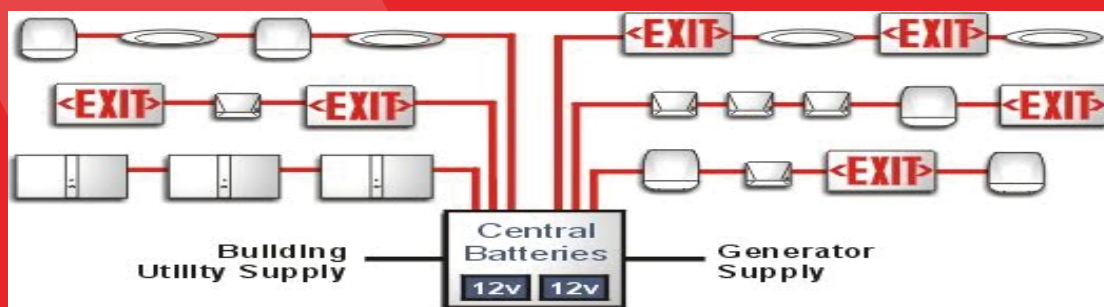
Central Battery & Central Monitoring
