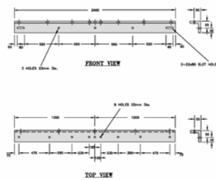
FIG.1: CROSSBAR - 1 100x100x12x4000mm L.G.
