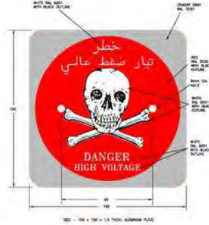
FIG.49: DANGER SIGN PLATE ALL DIMENSIONS ARE IN MILLIMETER
