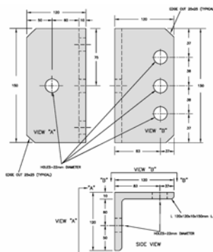
FIG. 5: EARTHWIRE SUSPENSION SUPPORT-1 120x120x10x150mm L.G. ALL DIMENSIONS ARE IN MILLIMETER
