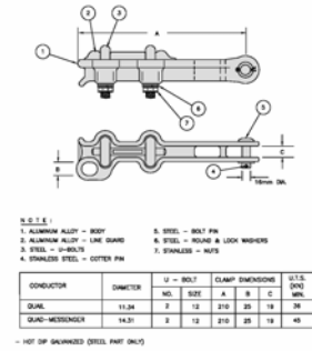
FIG.50: STRAIN CLAMP, STRAIGHT LINE DEADEND (2U-BOLT TYPE) ALL DIMENSIONS ARE IN MILLIMETER
