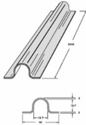
FIG.43: PVC GROUND WIRE GUARD
