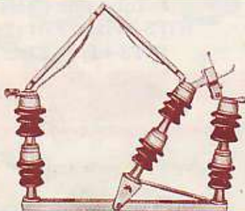
NTS-5 Double Stack Tilting Type 6 Insulators per phase
