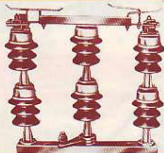
NTS-6 Double Stack Rotating Type 6 Insulators per phase
