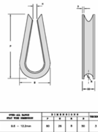
FIG.57: GUY THIMBLE ALL DIMENSIONS ARE IN MILLIMETER
