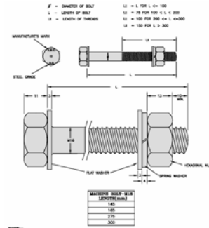
FIG.14: MACHINE BOLT - M16
