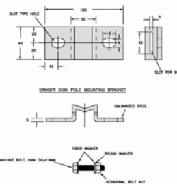
FIG.50: DANGER SIGN MOUNTING BRACKET
