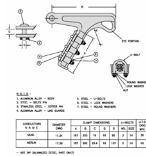
FIG.59: STRAIN CLAMPS, 3 U-BOLTS TYPE ALL DIMENSIONS ARE IN MILLIMETER
