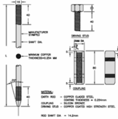
FIG.45: GROUNDING ROD 16mm DIA.
