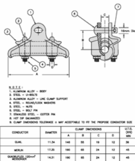
FIG.51: SUSPENSION CLAMP ALL DIMENSIONS ARE IN MILLIMETER
