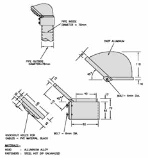
FIG.58: SERVICE ENTRANCE HEAD FOR MAST 75mm DIA. STEEL PIPE ALL DIMENSIONS ARE IN MILLIMETER
