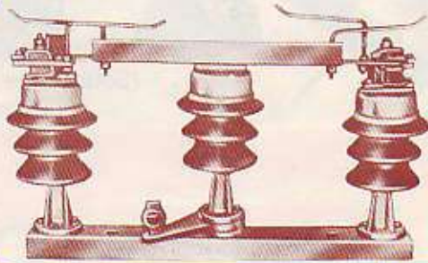
NTS-4 Centre Post Rotating 3 Insulators per phase
