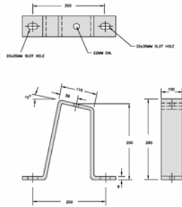
FIG. 8: HORIZONTAL INSULATOR MOUNTING BRACKET ALL DIMENSIONS ARE IN MILLIMETER
