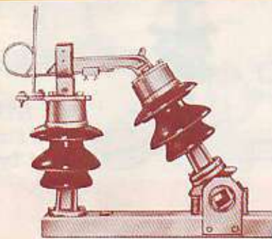
NTS-1 Tilting Type 2 Insulators per phase
