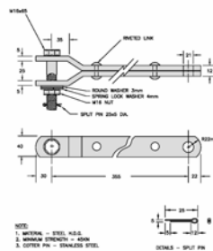
FIG.21: CLEVIS EYE EXTENSION
