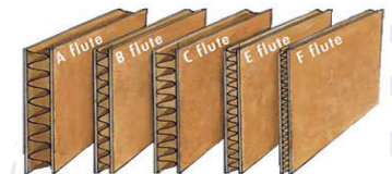
Flute Types
