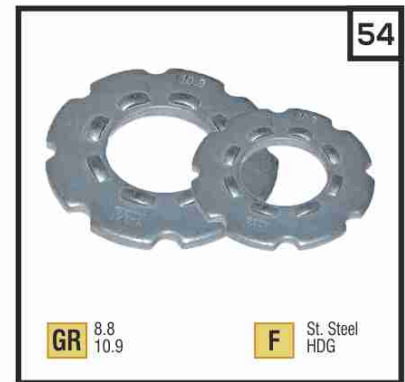
LOAD INDICATING WASHER ASTM F959M
