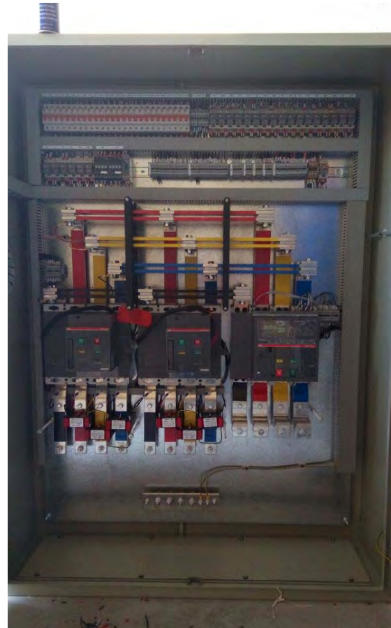
Synchronising Panels
